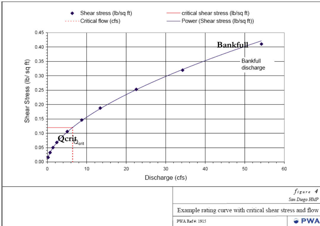
Figure 5-4. Example of a Rating Curve with Critical Shear Stress for Medium Sized Gravel.
