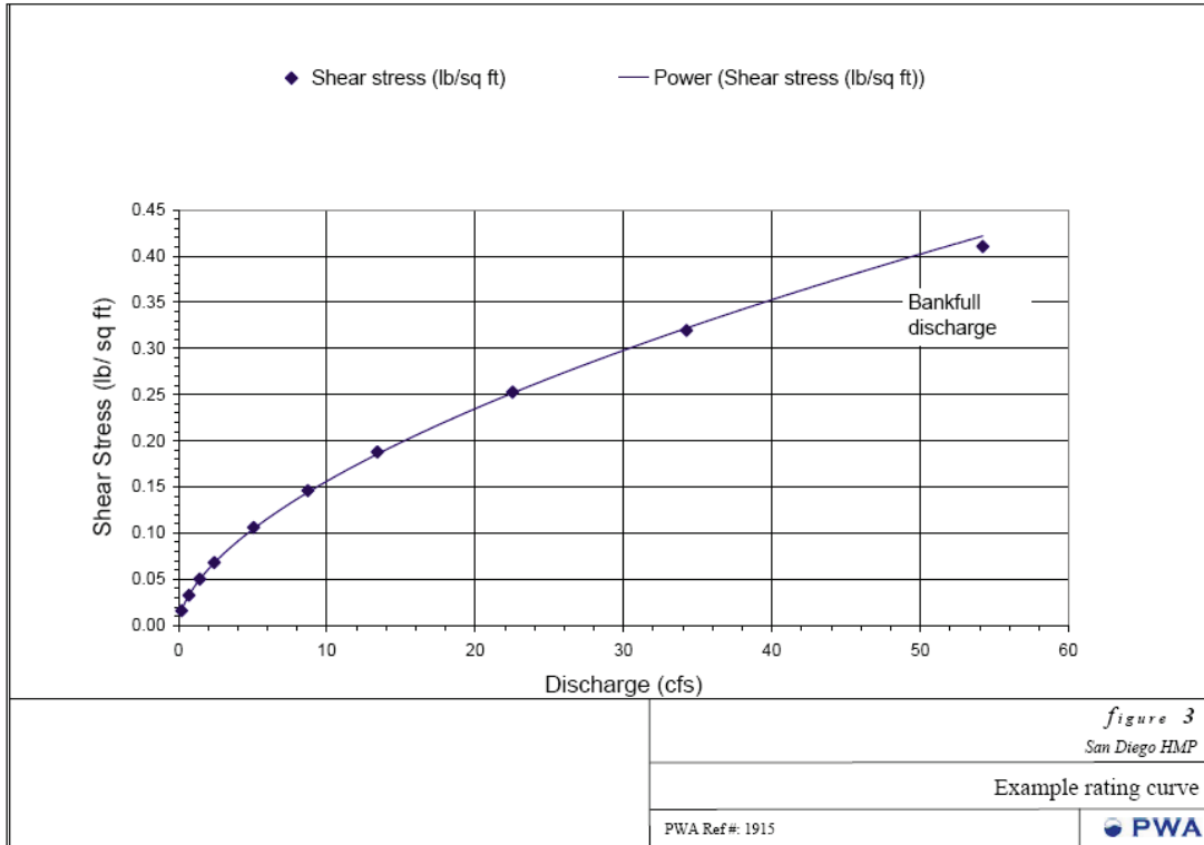
Figure 5-3. Shear Stress Rating Curve for an Example Channel (0.6%, 14 Feet Wide, 1.3 Feet Deep). These curves were created for 36 different combinations of channel characteristics.
